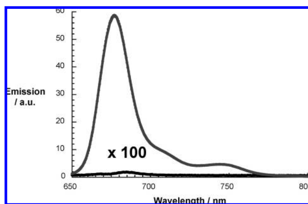
Figure 6. Steady-state fluorescence spectra of ZnPc reference (gray spectrum) and SWNT-ZnPc 5 (black spectrum) in THF at room temperature with matching absorption at the excitation wavelength (i.e., 650 nm). The spectra were not corrected for different ground state absorption at the excitation wavelength.
