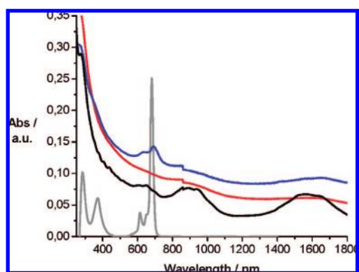
Figure 5. Absorption spectra of ZnPc 1 (gray) in NMP and p -SWNTs 6 (black), f -SWNTs 8 (red), and SWNT-ZnPc conjugates 5 (blue) in SDS (1.2 CMC)/ D 2 O.
