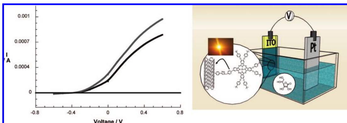
Figure 8. I–V characteristics of SWNT-ZnPc 5 under white light illumination, gray line, and in the dark, black line. Three-electrode setup, 0.1 M Na 3 PO 4 , 1 mM sodium ascorbate, N 2 purged. Voltages measured versus a Ag/AgCl reference electrode (0.1 M KCl). On the right: schematic representation of the photoelectrochemical cell used for the measurements.
